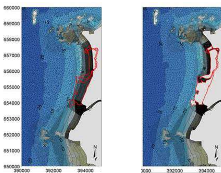
Figure 5.8 Model area for detailed sediment modelling; existing condition (left) and with Project (right). Unstructured mesh used for the Tg Aru fine local hydrodynamic model that extend past Lok Kawi
