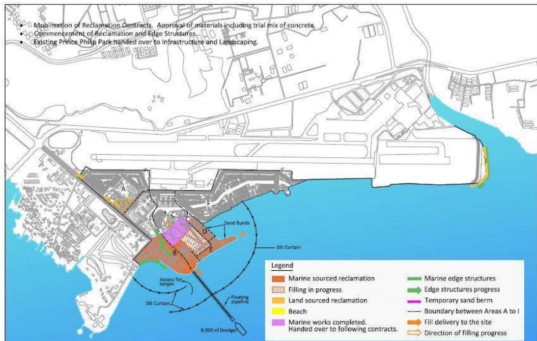
Figure 2.11 Drawing No 101 - works begin at Fisherman's wharf area with land fill material being used at Area A and the access road to the south of the airport
