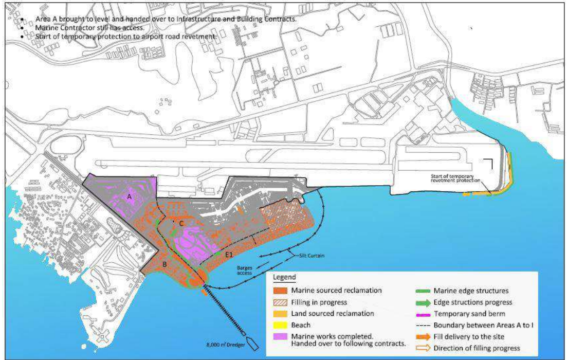
Figure 2.12 Drawing No 102 - works progressing south with Prince Phillip Park and the first section of beach filled
