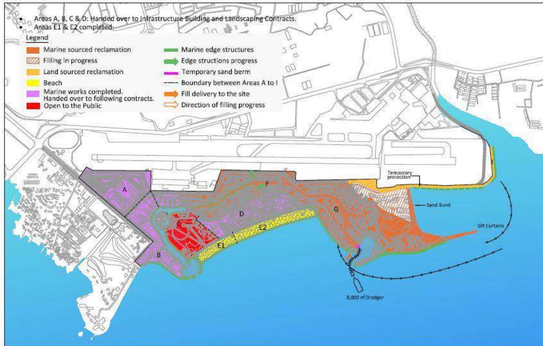
Figure 2.14 Drawing No 104 - Prince Phillip Park open to the public and all the beach sand placed for potential opening of the beach, main works continuing south.
