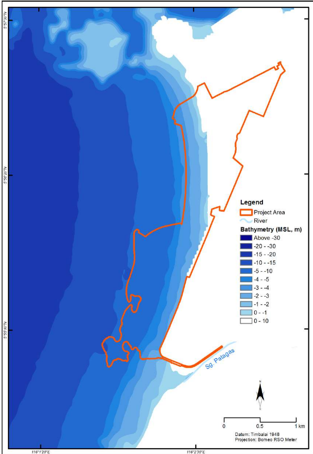
Figure 3.1 Bathymetry at Project site.
